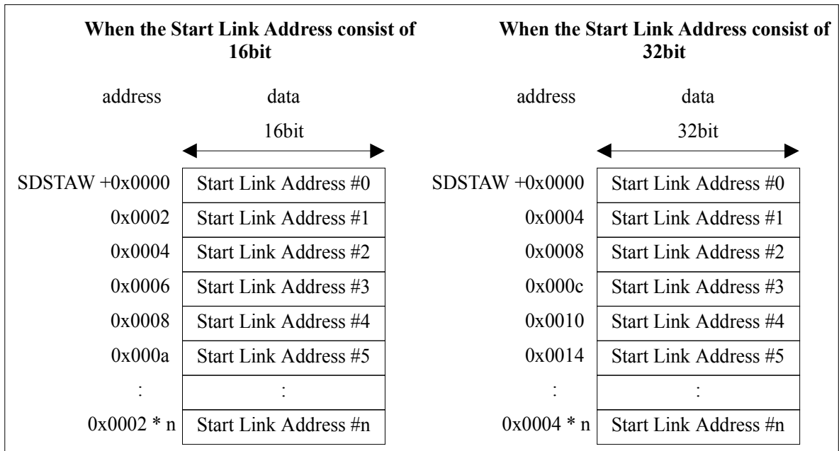
Fig. 2-10 Start Link Address Table Format
